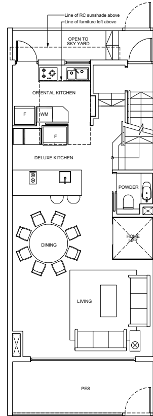
1ST STOREY
